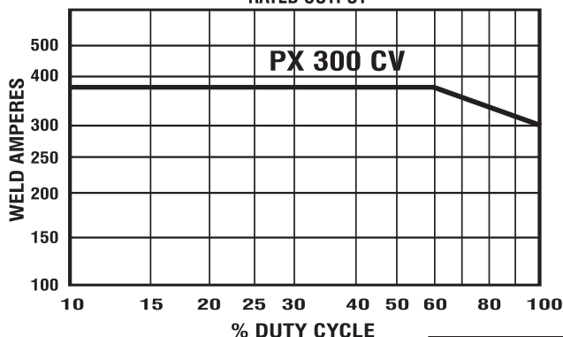
DUTY CYCLE RATED OUTPUT
